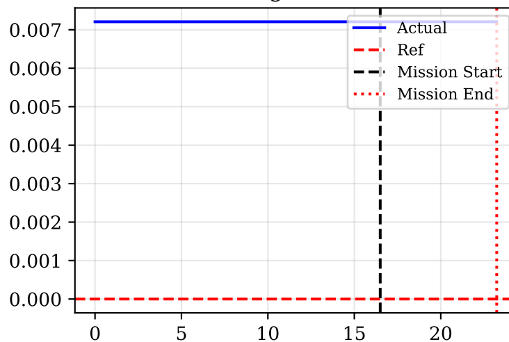
Norm Omega Error [rad/s]
