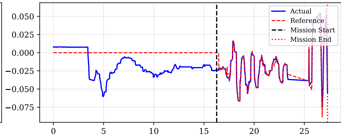
Pitch [rad]
