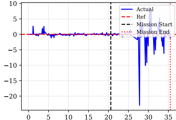
Angular Acc Z [ \text{rad/s}^2 ]
