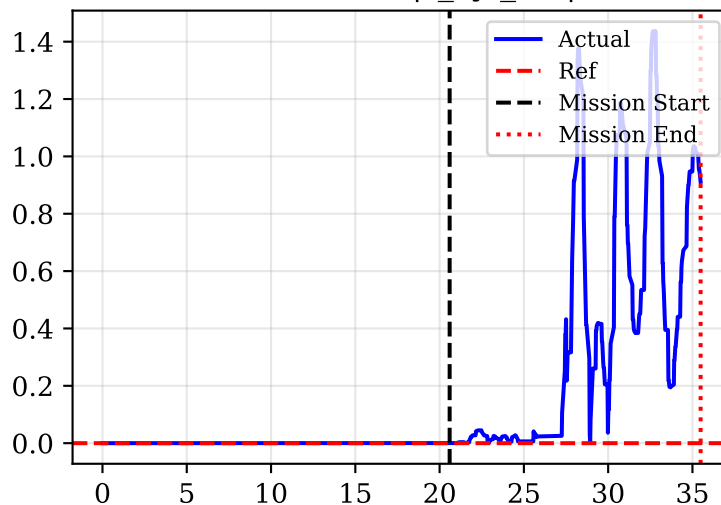
Yaw Error [ \gamma_{err} ] [rad]
