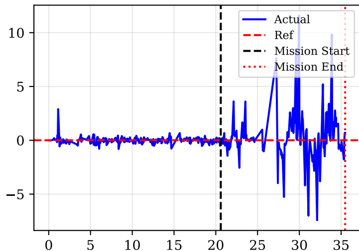
Angular Acc X [ \text{rad/s}^2 ]
