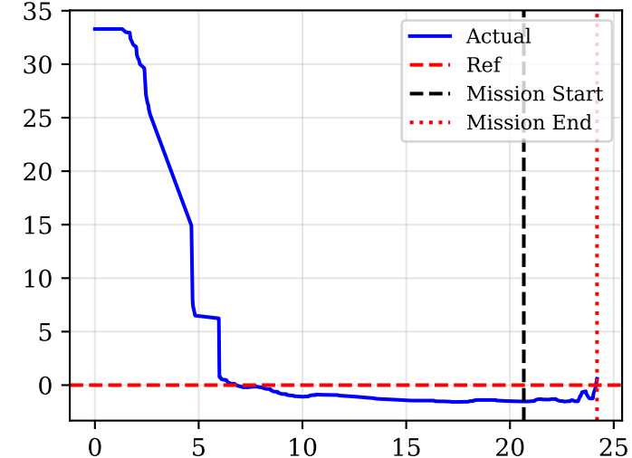
Force Z [N]
