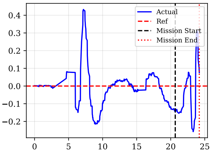
Force X [N]
