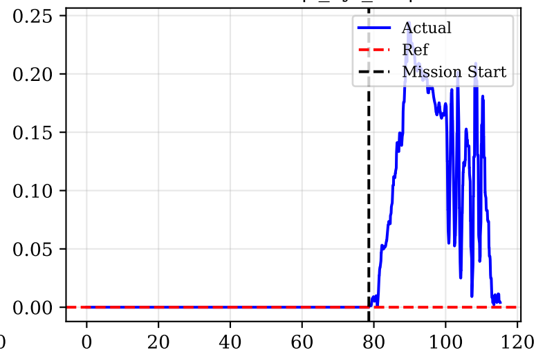
Yaw Error |yaw_err| [rad]
