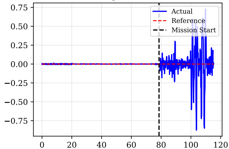
Omega X [rad/s]
