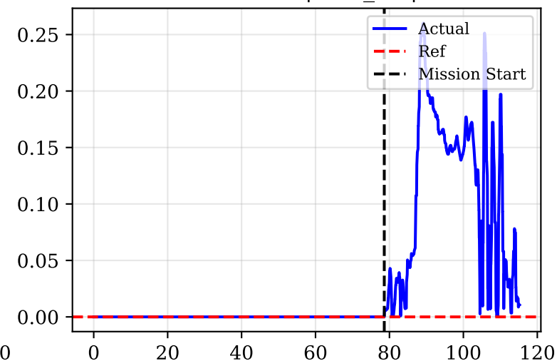
Norm Roll/Pitch Error
