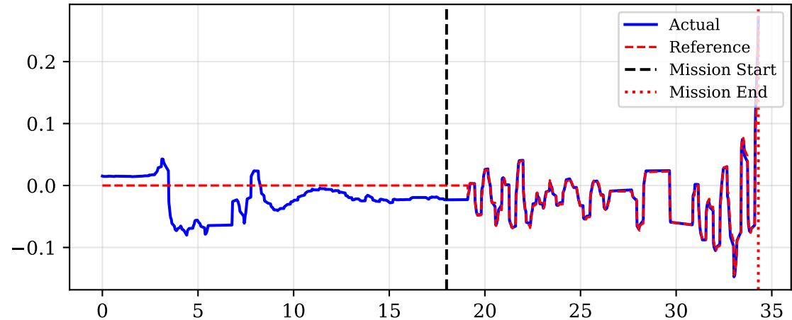
Pitch [rad]
