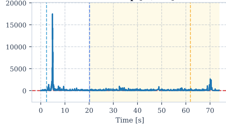
Norm Snap [m/s^4]
