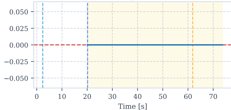
Vert. FoV Violation s_{fov,v} [deg] (half-FoV=29°)
