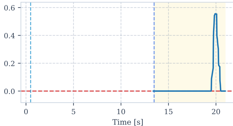
Distance Violation s_r [m] ( r_{min}=1.0 m)
