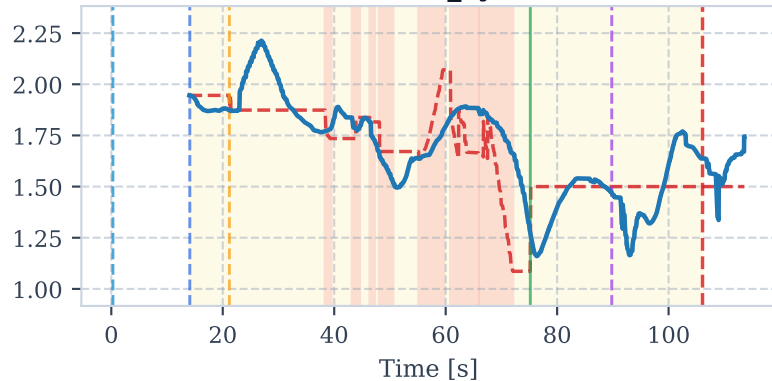
Distance r_{cyl} [m]
