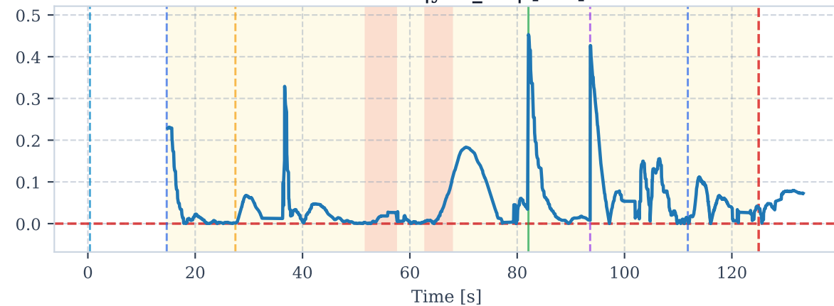
Yaw Error |\gamma_{err}| [rad]
