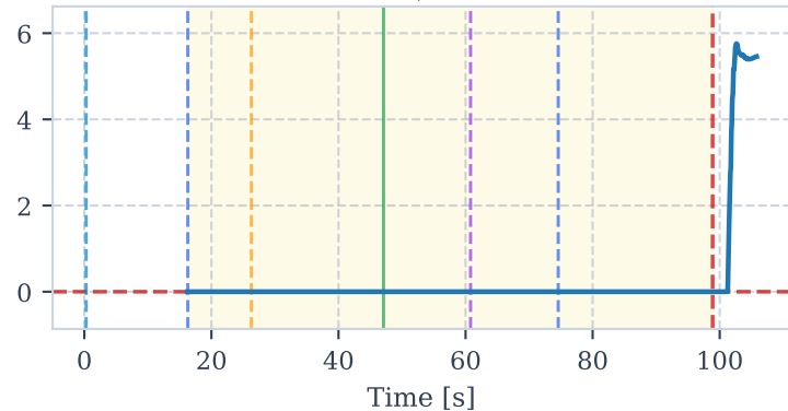
Vert. FoV Violation s_{fov,v} [deg] (half-FoV=29°)
