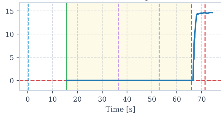
Vert. FoV Violation s_{fov,v} [deg] (half-FoV=26°)
