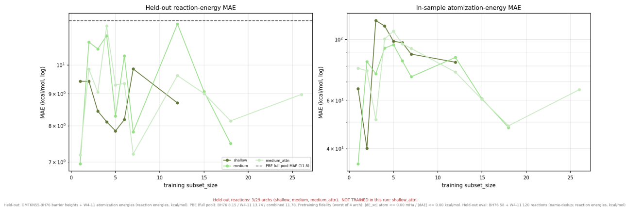
Figure 17: Learning curves: held-out reaction-energy MAE against training subset size, one line per architecture, with the full-pool PBE reference dashed. Left panel held-out, right panel in-sample.
