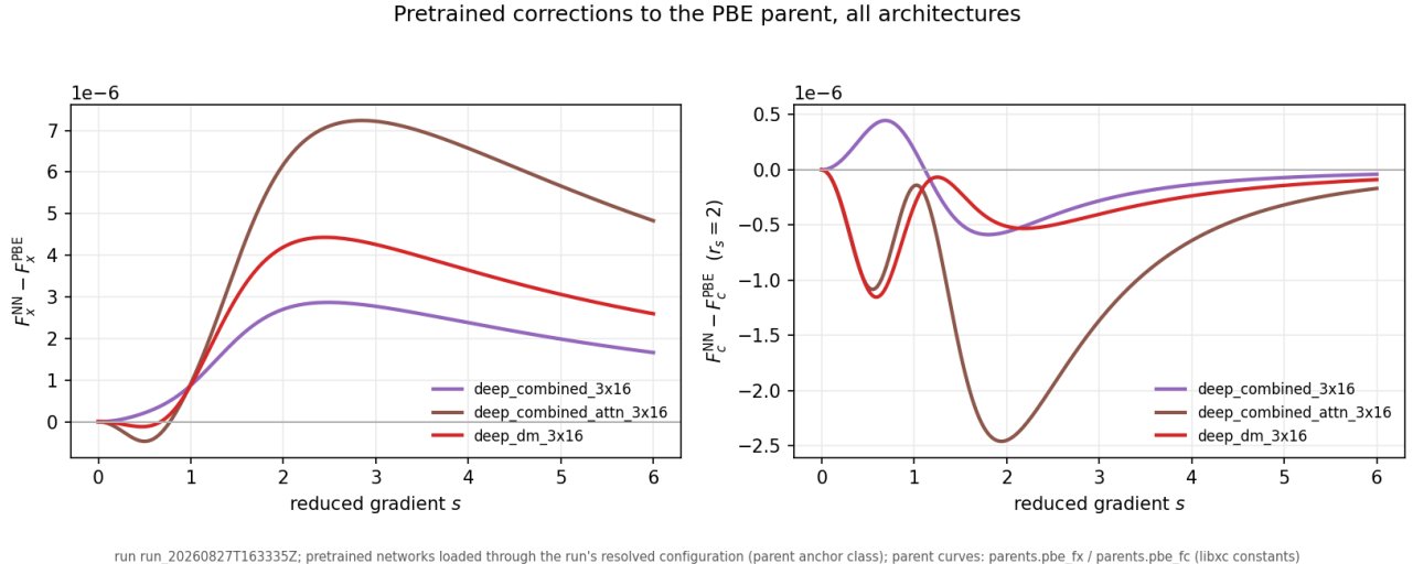
Figure 21: Anchored (v6 G3) pretrained corrections to the PBE parent for the dm-descriptor family (deep_dm_3x16, deep_combined_3x16, deep_combined_attn_3x16), both channels.
