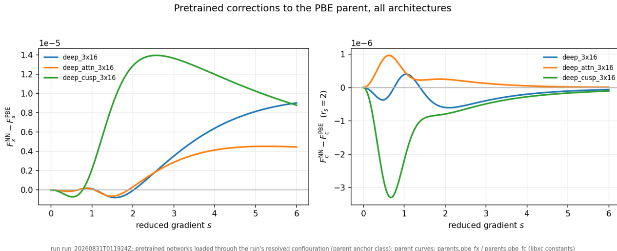
Figure 20: Anchored (v6 G2a) pretrained corrections to the PBE parent for the core trio (deep_3x16, deep_attn_3x16, deep_cusp_3x16), both channels.
