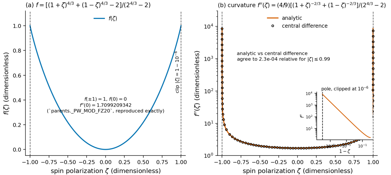
PW92 spin interpolation and the clipped curvature pole
