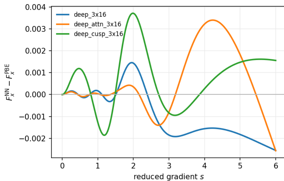
Pretrained corrections to the PBE parent, all architectures
