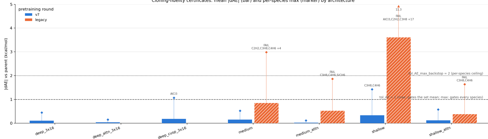
Cloning-fidelity certificates: mean |dAE| (bar) and per-species max (marker) by architecture
