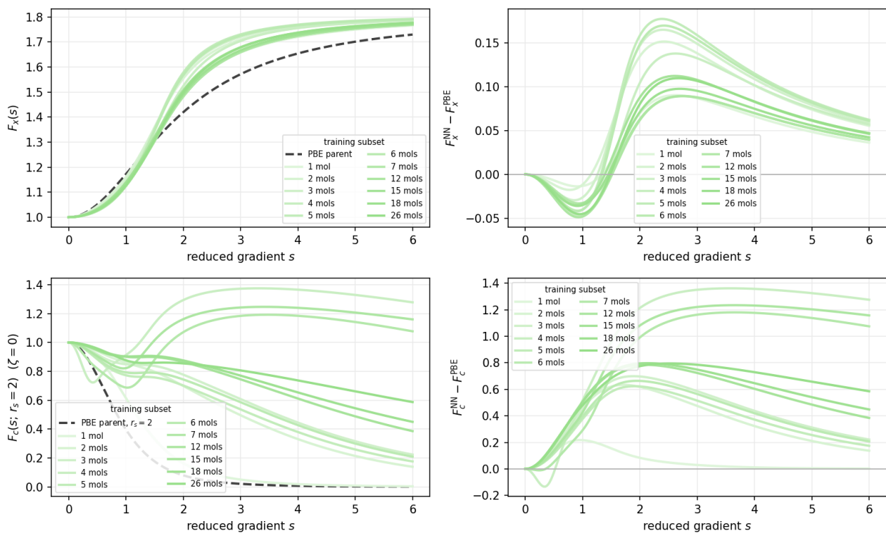
medium: trained networks against the PBE parent
