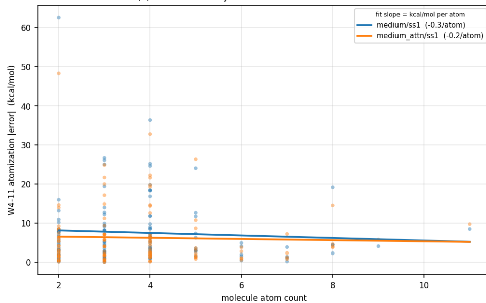
(a) Size-consistency: atomization error vs molecule size
