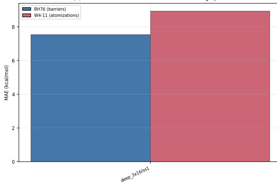
(b) Barriers vs atomizations -- the cancellation fingerprint
