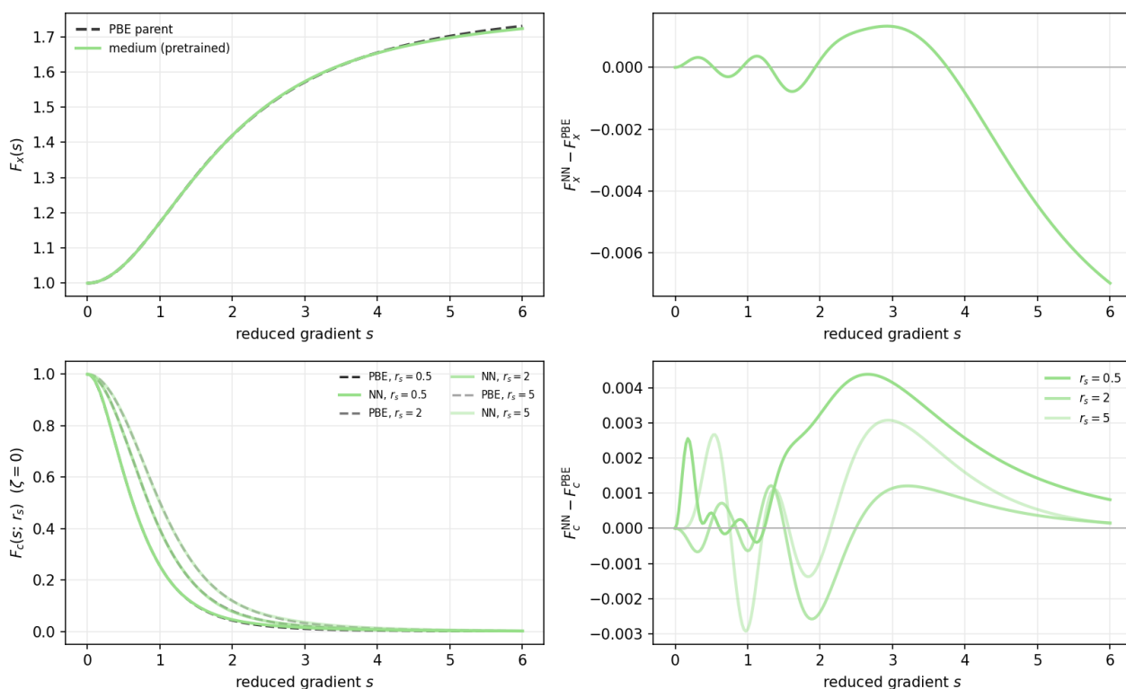
medium: pretrained network against the PBE parent
