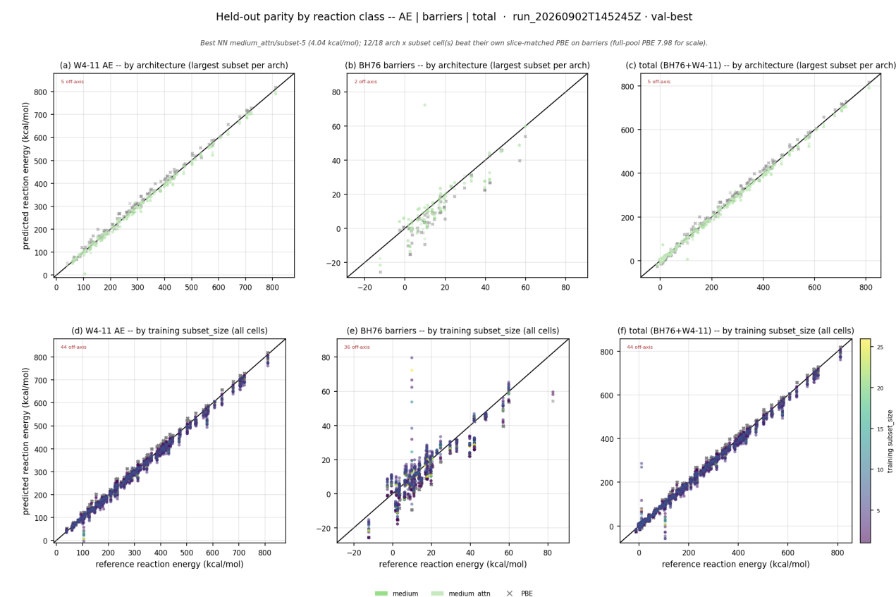
Fig. 5.3 Parity of the predicted against the reference reaction energy, one point per held-out reaction, by reaction class in three columns (W4-11 atomizations, BH76 barriers, both together). The top row draws each architecture at its largest subset; the bottom row pools every cell and colors the points by subset size; PBE on the same reactions is drawn as grey crosses in every panel and the diagonal is the exact line. Each panel prints the number of points outside its axis range. The atomization column spans 0 to 800 kcal/mol; at that scale the networks and PBE lie on the diagonal (5 points off-axis in the top panel, 44 in the bottom one, the largest of them the one-molecule cells' errors of 60 kcal/mol on the smallest molecules, Fig. 5.8), and the per-reaction errors of a few kcal/mol that the tables report are not resolved. The barrier column spans -25 to 85 kcal/mol. In the top panel the largest-subset cells (medium at 26, medium_attn at 7) scatter around the diagonal with residuals up to about 10 kcal/mol and one medium_attn barrier predicted at 72 kcal/mol against a reference of 10, while the PBE crosses sit mostly below the diagonal between references of 0 and 20 kcal/mol; in the bottom panel the two-to-six-molecule cells (the darkest colors) spread widest, the reference barrier of 10 kcal/mol being predicted from -5 to 80 kcal/mol across cells, with 36 points off-axis.
