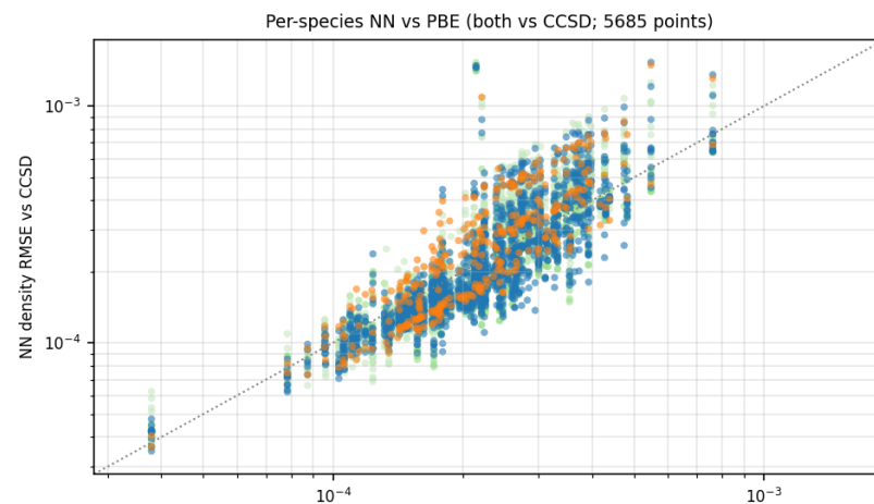
PBE density RMSE vs CCSD
