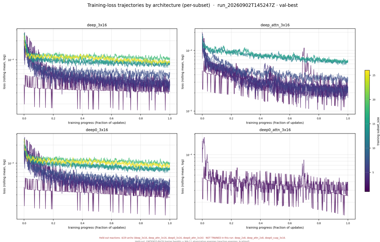
Fig. 4.2 The total training loss per cell as a rolling mean over the group updates (log axis against the fraction of the run’s updates; the first panel of Fig. 4.1 on the update rather than the epoch axis), one panel per architecture, one curve per subset size. The curves are the quantity stepped; the fall between the first and the last five percent of the updates is the “loss fall” column of the table in Sec. 4.5 (1.2 to 5.1 over the 33 cells). The deep_3x16 panel separates into the two plateaus of Fig. 4.1 (1e-4 for the cells from twelve molecules upward, 3e-5 to 5e-5 below); the one-molecule curve alternates between two levels from update to update. The deep_attn_3x16 panel shows transient rises near 45 and 70 percent of the run in the one- and two-molecule cells, the spikes of the potential and density channels around epochs 85 to 105 in Fig. 4.1.
