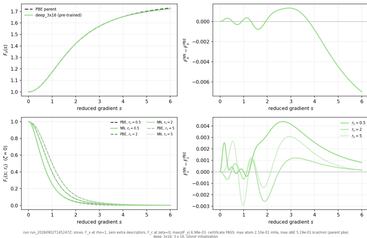
deep_3x16: pre-trained network against the PBE parent
