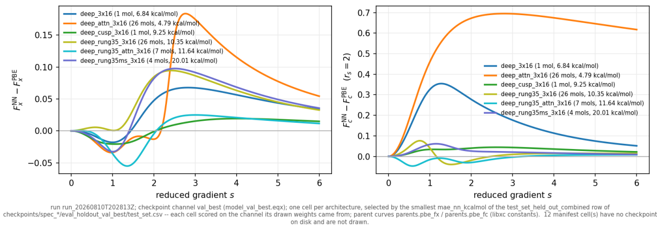
Figure 13: Optimized (validation-best) enhancement-factor differences from PBE, unanchored v4gga, one cell per architecture at its largest completed subset size.
