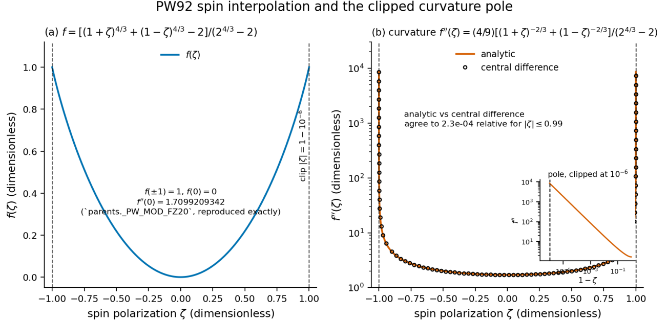
Figure 3: PW92 spin interpolation f(\zeta) and its curvature. Left: the interpolation, with the production clip at |\zeta| = 1 - 10^{-6} marked. Right: f''(\zeta) , analytic against a central difference, on a log scale, with the pole resolved in the inset.
