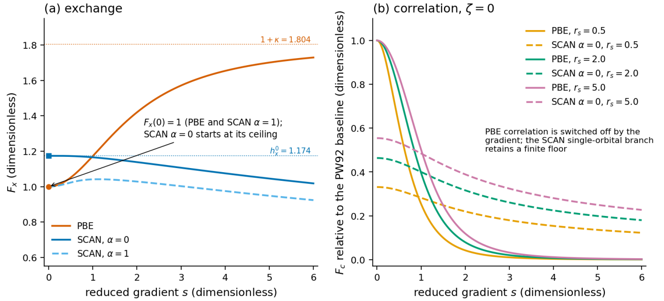
Figure 2: Parent enhancement factors at libxc constants. Left: exchange, PBE against SCAN at \alpha = 0 and \alpha = 1 , with the two ceilings marked. Right: correlation relative to the PW92 baseline at three densities, \zeta = 0 .
