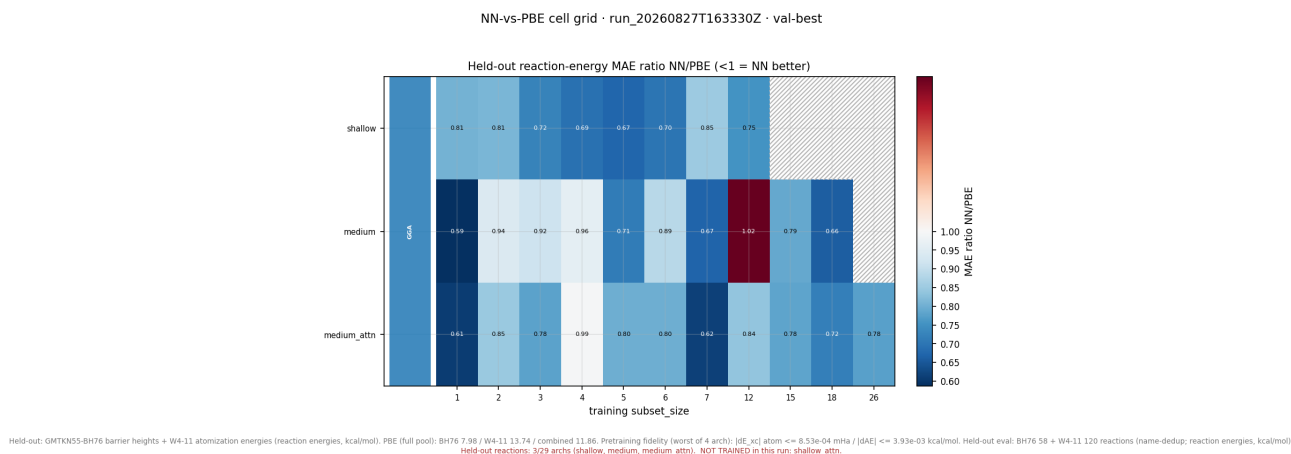
Figure 18: NN-against-PBE cell grid: the ratio of held-out reaction-energy MAE, architecture by subset size, diverging about 1.0. Blue is better than PBE; missing cells are hatched.
