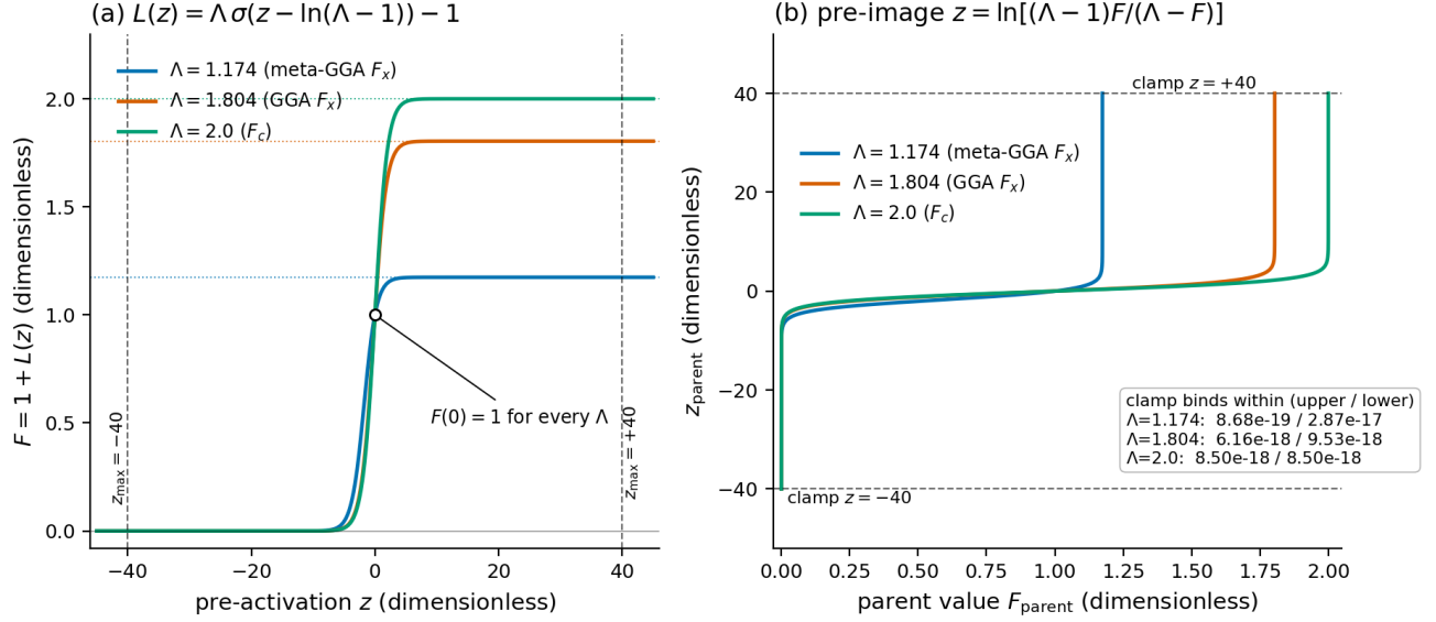
Figure 1: Bounded map and its pre-image. Left: F = 1 + L(z) for the three limits in use, with the pre-image clamp at z = \pm 40 marked. Right: the inverse z = \ln[(\Lambda - 1)F/(\Lambda - F)] , annotated with the distance from each bound inside which the clamp binds.
