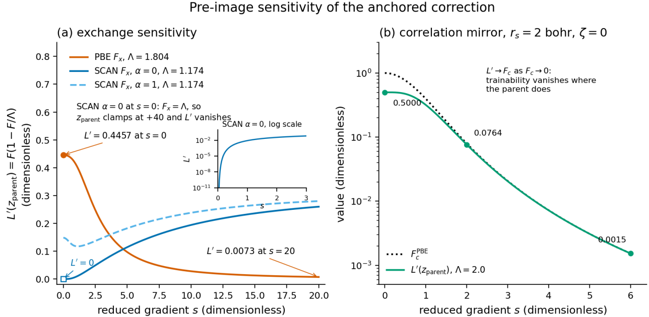
Figure 16: Pre-image sensitivity of the anchored correction. Left: exchange, L'(z_{\text{parent}}) against s for the PBE parent at \Lambda = 1.804 and the SCAN parent at \Lambda = 1.174 for both indicator slices, with the SCAN \alpha = 0 case on a log inset. Right: the correlation mirror at r_s = 2 , \zeta = 0 , showing L' tracking F_c down to zero.
