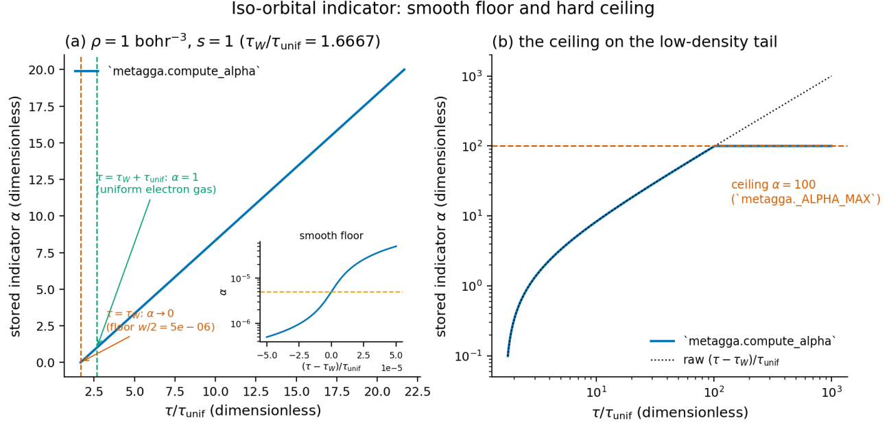
Figure 4: Iso-orbital indicator: smooth floor and hard ceiling. Left: the stored \alpha against \tau/\tau_{\text{unif}} at \rho = 1 and s = 1 , with the single-orbital and uniform-gas points marked and the smooth floor resolved in the inset. Right: the same on log axes, showing the ceiling truncating the low-density tail.
