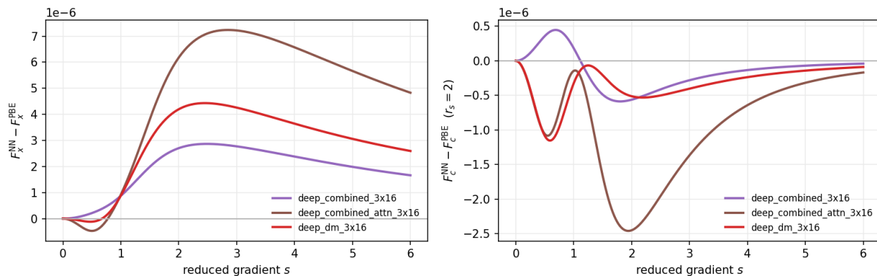
Figure 21: Anchored (v6 G3) pretrained corrections to the PBE parent for the dm-descriptor family (deep_dm_3x16, deep_combined_3x16, deep_combined_attn_3x16), both channels.
