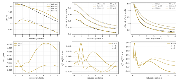
deep0_cusp_mgga_3x16: pre-trained network against the SCAN parent
