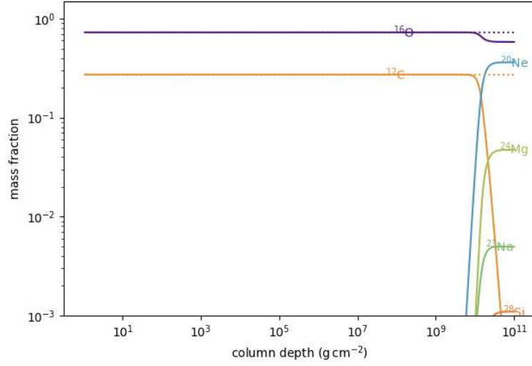
Figure 2: Composition of elements within stellar (compact) object as a function of column depth.
