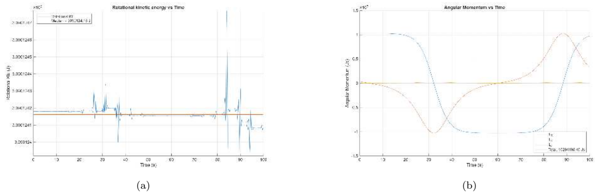
Figure 4: Rotational kinetic energy (left) and angular momentum (right). Rotational kinetic energy is essentially constant with noise due to small errors in the numerical integration. Notice the scale of the y-axis.
