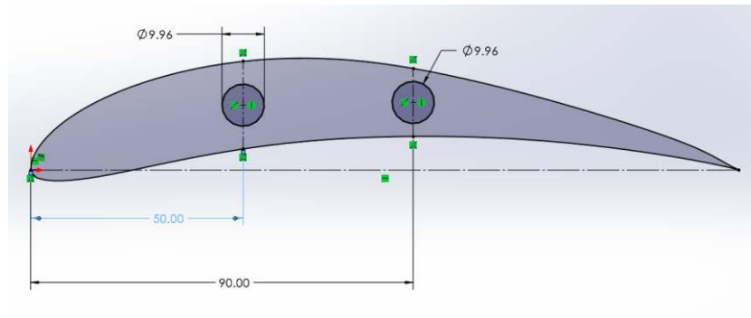
Figure 4: CAD sketch of aerofoil section
