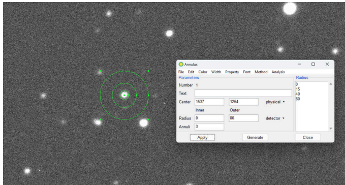
Figure 3: First image taken of CoRoT-1 with an annulus over the target star.
