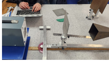
(a) Polarisation apparatus showing metal grate placed between microwave source and detector.
