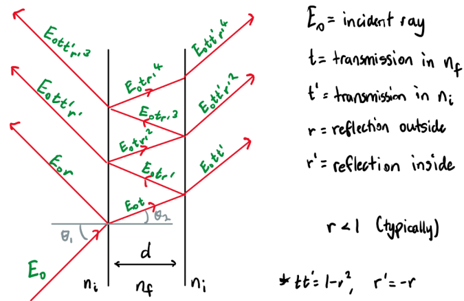
Figure 8: A diagram of multiple beam interference seen in Fabry-Perot interferometry. Keep in mind that in our experiment we did this along only a single dimension, not as shown.
