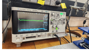
(b) Digital oscilloscope used for intensity measurements.
