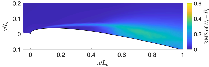
Figure 5: The root-mean-squared of the mean-subtracted velocity field.
