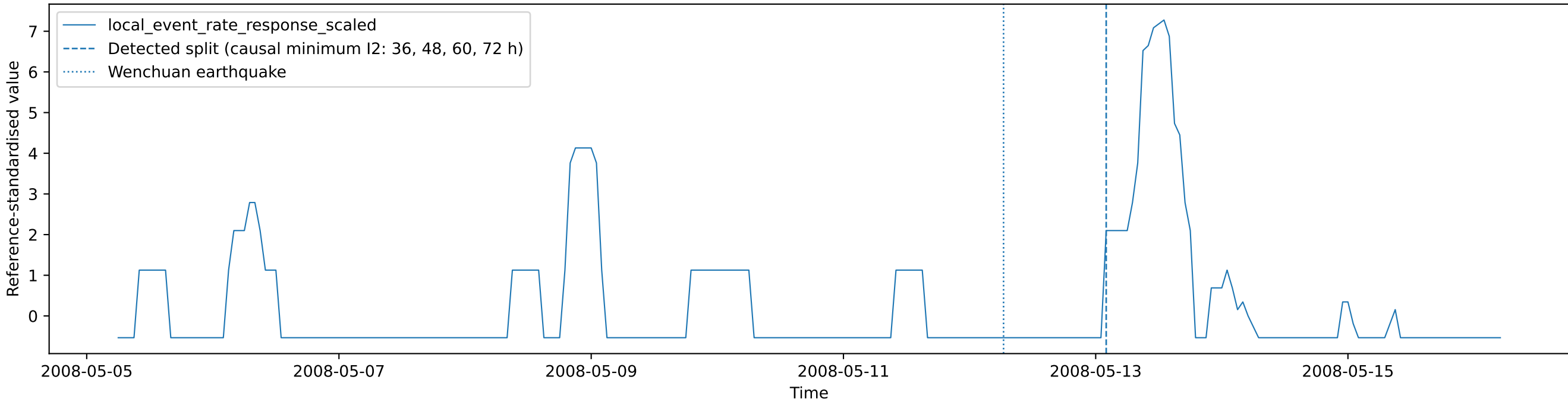
local_event_rate_response_scaled: data-selected split partitions
