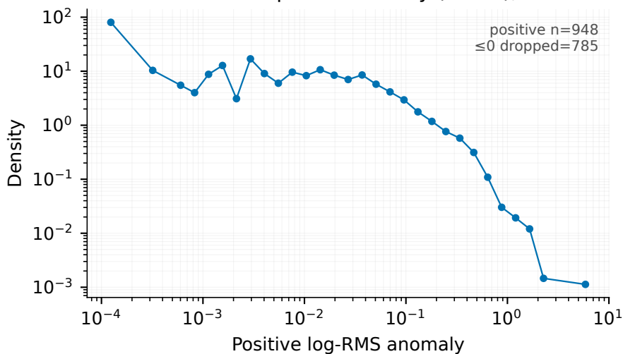
SO 2 flux
