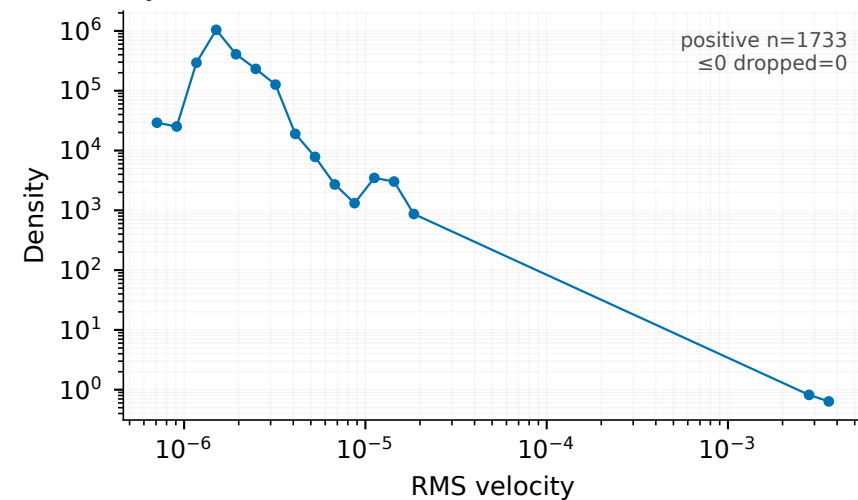
Positive tremor-response anomaly (Effect), 5-15 Hz
