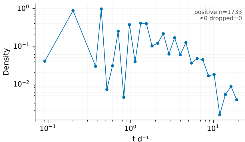
SO 2 flux
