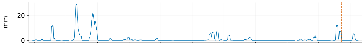
12-hour rainfall sum
