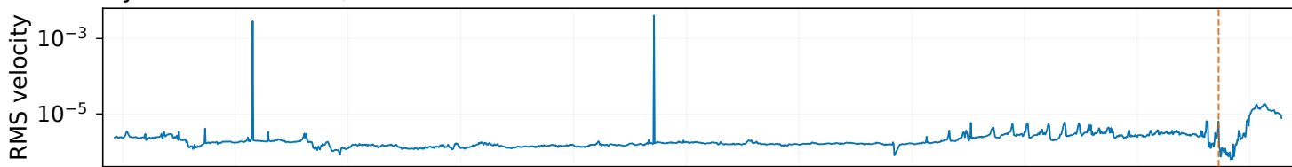
Hydrothermal RMS, 2-5 Hz
