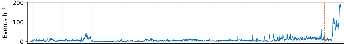
STA/LTA event rate, 2-5 Hz
