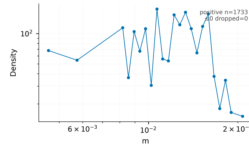
GNSS deformation
