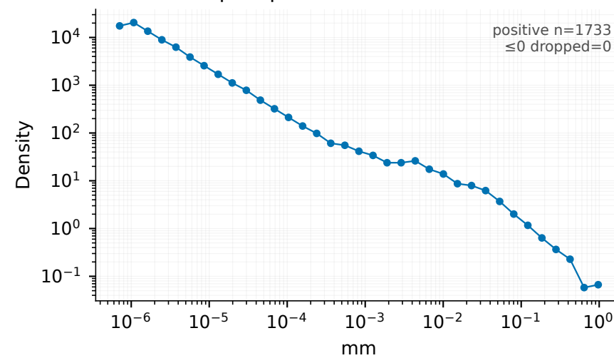
GNSS deformation
