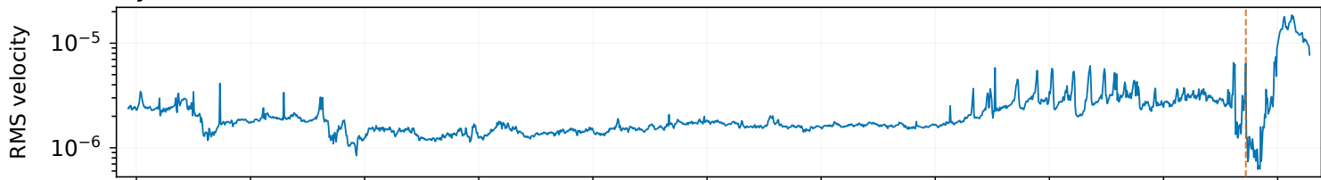
Hydrothermal RMS, 2-5 Hz
