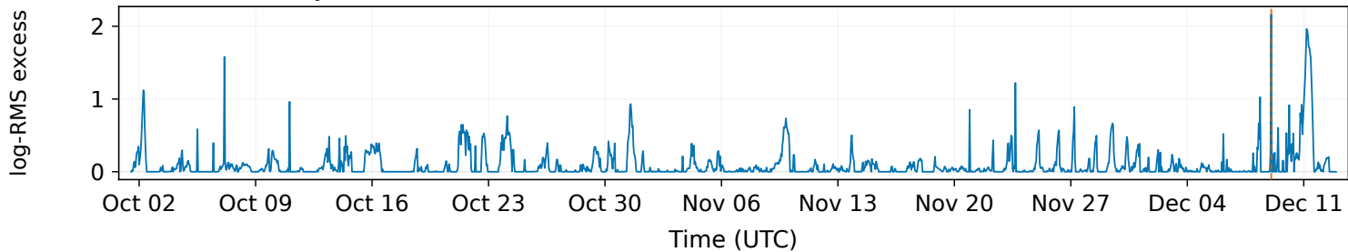
Tremor anomaly (Effect), 5-15 Hz
