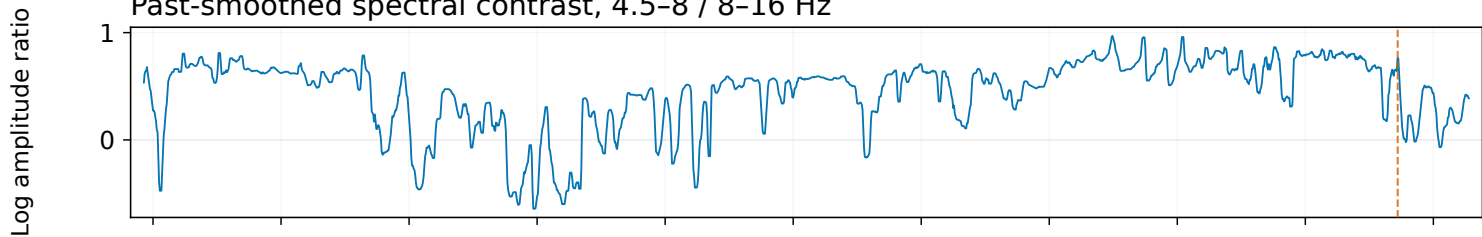
Past-smoothed spectral contrast, 4.5-8 / 8-16 Hz
