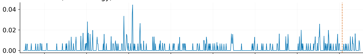
Etna tremor/state energy, 0.80–2.30 Hz
