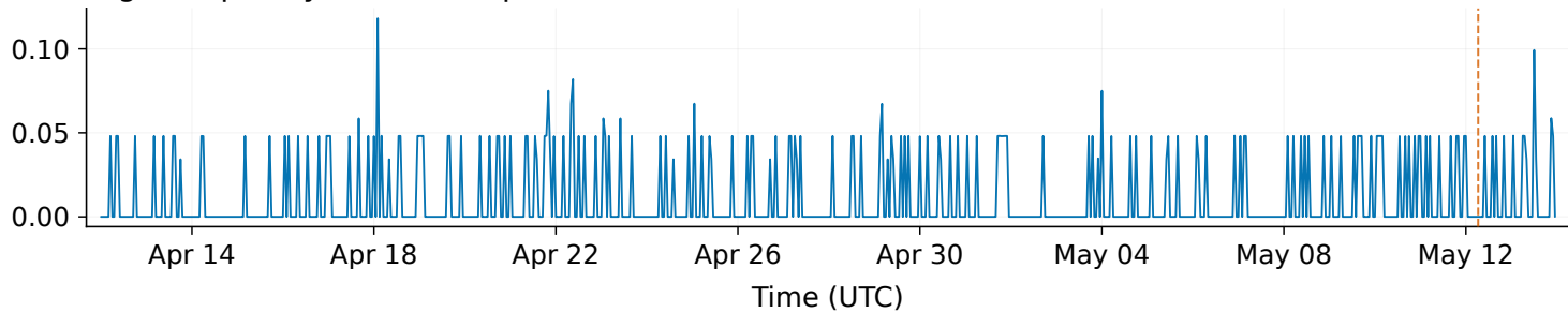
High-frequency seismic response (Effect), 4–8 Hz
