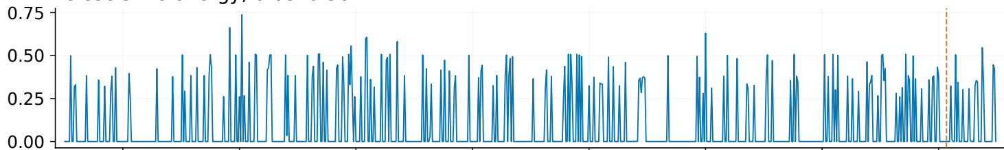
Teleseismic energy, 0.03–0.30 Hz
