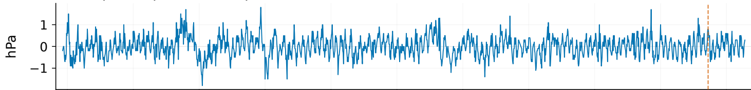
Atmospheric pressure drop
