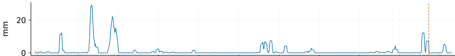
12-hour rainfall sum
