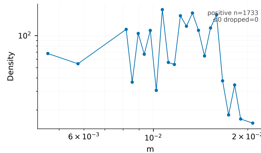
GNSS deformation
