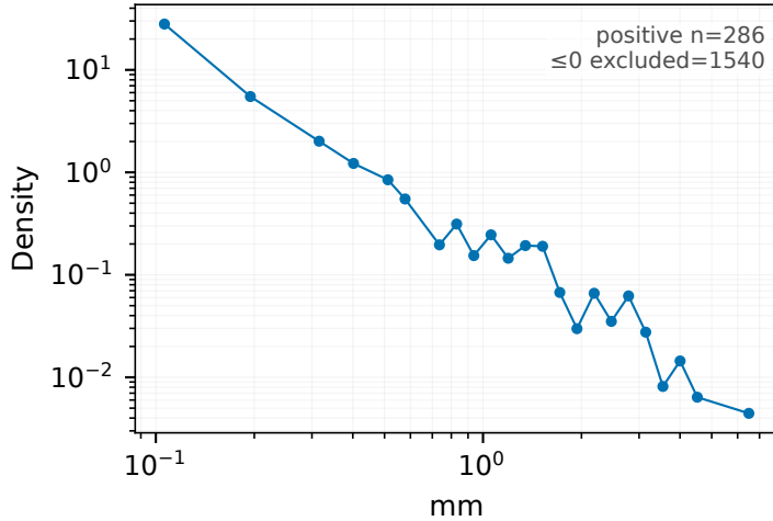
Hourly precipitation
