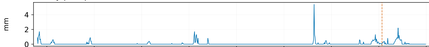
Hourly precipitation
