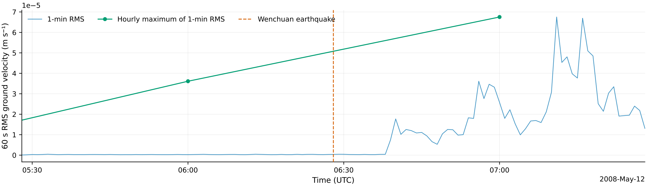
ME01: hourly aggregation of response-corrected ground motion
