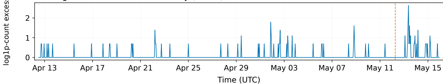
Catalogue local event-rate anomaly (Effect)
