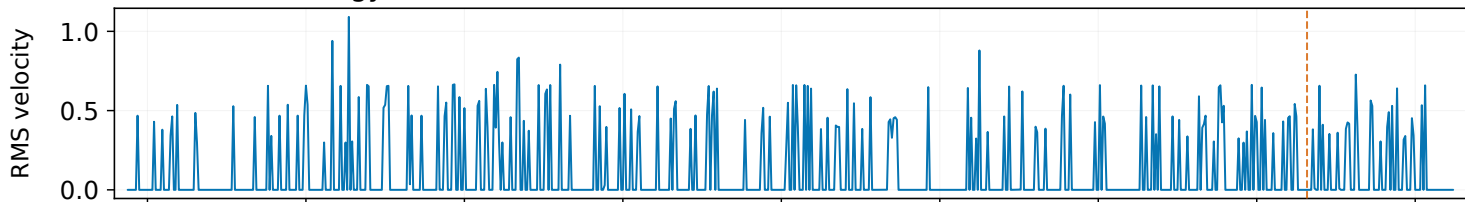
Teleseismic energy, 0.03-0.30 Hz
