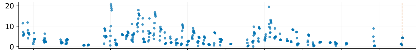
SO 2 flux
