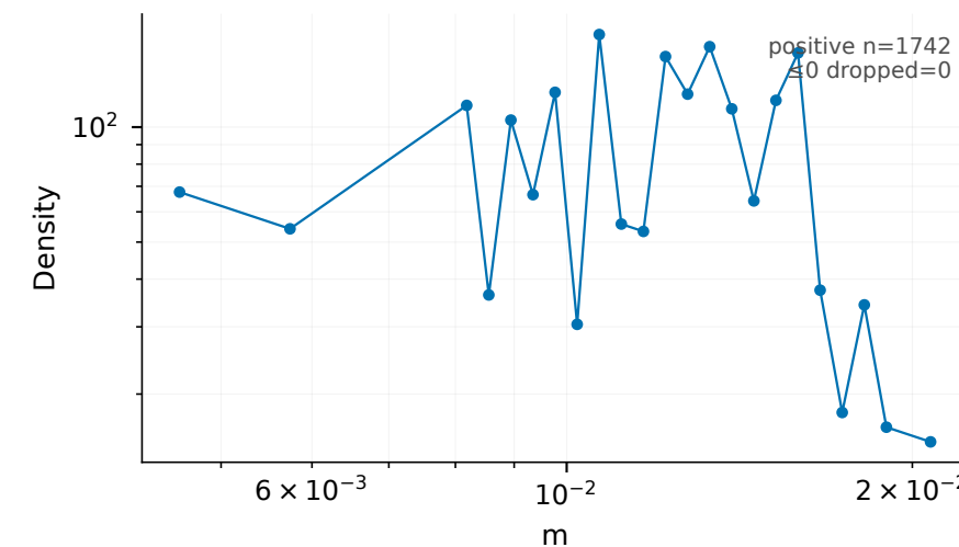
GNSS deformation
