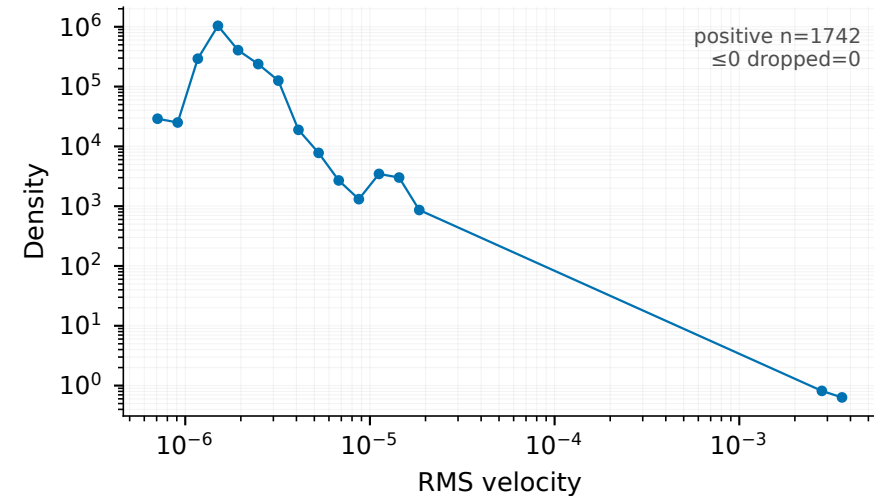
Tremor response RMS (Effect), 5-15 Hz
