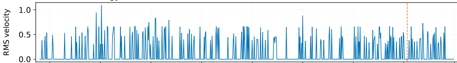
Teleseismic energy, 0.03-0.30 Hz
