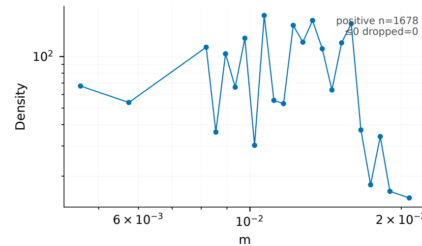
GNSS deformation
