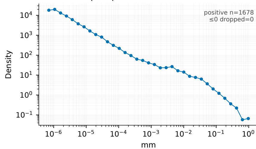
GNSS deformation
