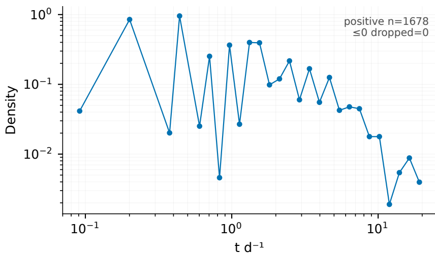
SO 2 flux
