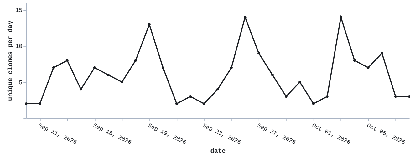
Unique cloners
