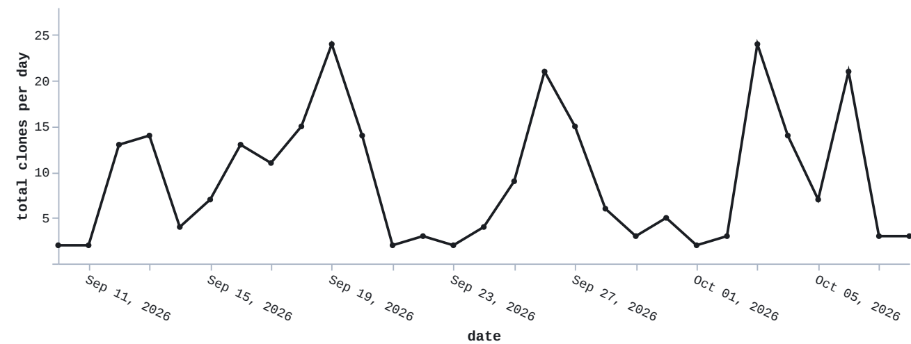
Total clones
