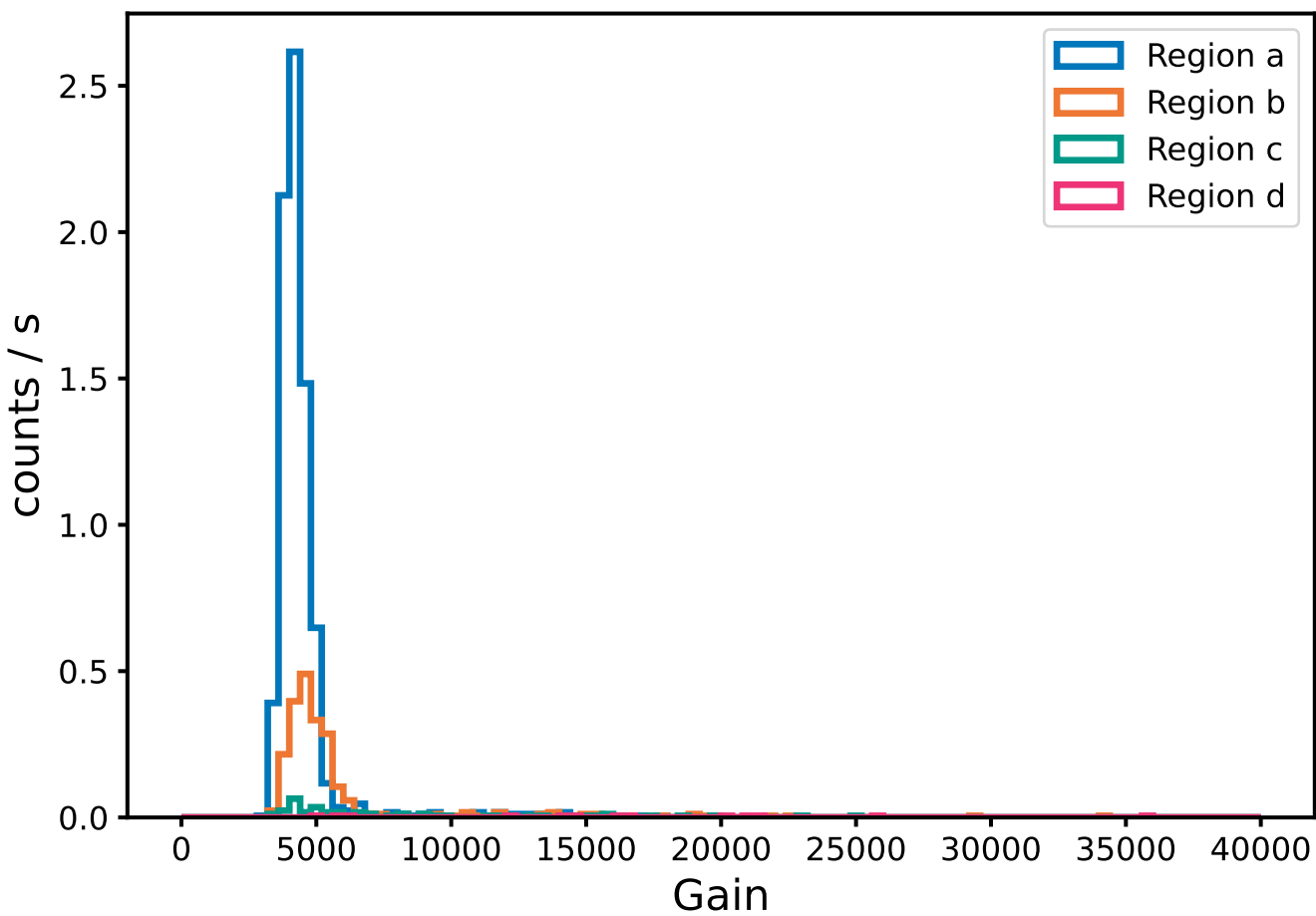
Dataset: Recent
