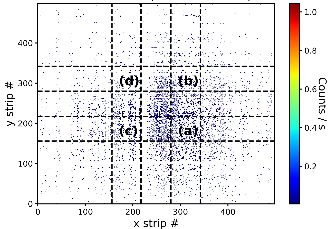
Dataset: 750V (lower threshold)
