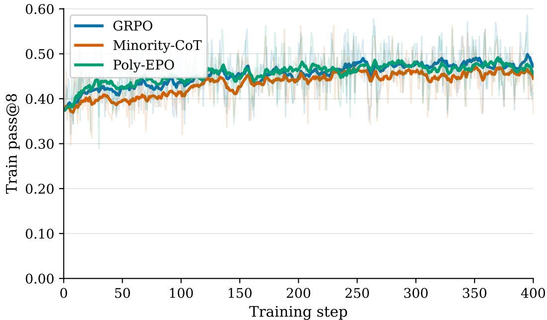
Training Accuracy (pass@8) — 400 Steps
