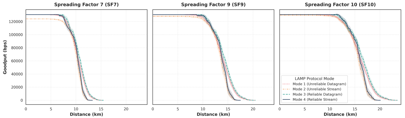
Fig. 6. Effective application-layer throughput (Goodput in bps) across Spreading Factors and LAMP operational modes in LoS. Shaded ribbons denote 95% confidence intervals across 50 Monte Carlo trials.
