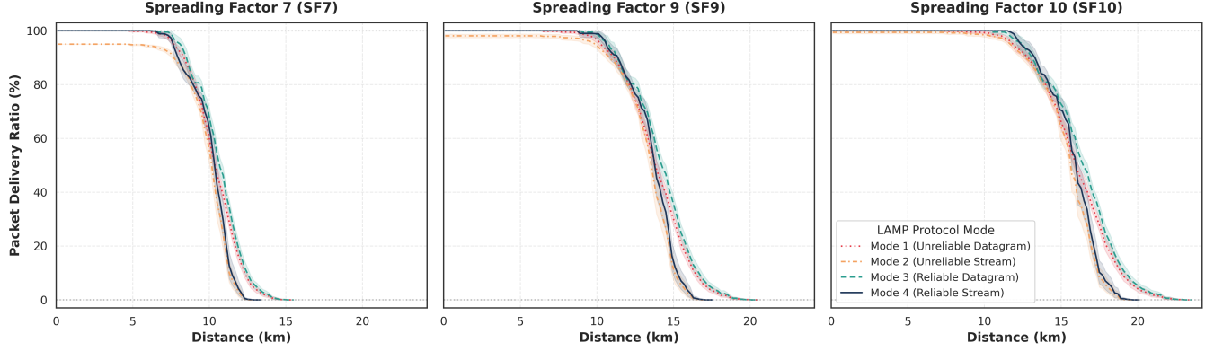
Fig. 5. Packet Delivery Ratio ( PDR_{app} %) as a function of distance across Spreading Factors (SF7, SF9, SF10) in Line-of-Sight (LoS) propagation. Solid lines denote mean delivery rates across 50 Monte Carlo trials; shaded ribbons represent 95% confidence intervals.
