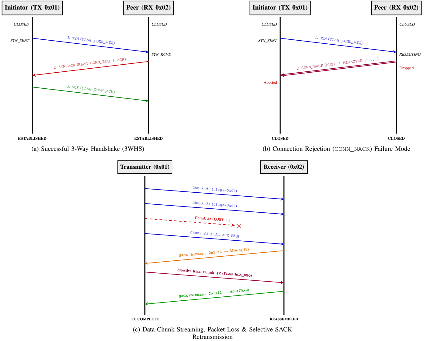
Fig. 3. Sequence interaction flows for connection establishment, CONN_NACK rejection, and SACK-driven selective retransmission under frame loss.
