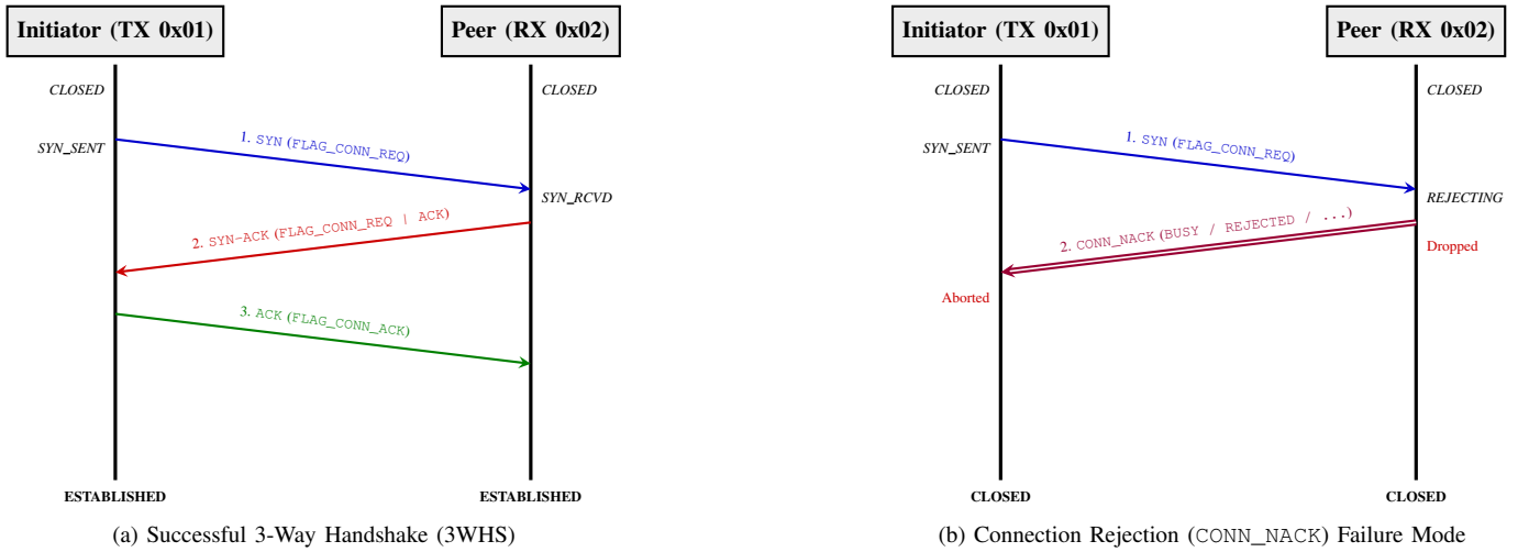
Fig. 3. Sequence interaction flows for successful 3-Way Handshake and CONN_NACK rejection failure modes.
