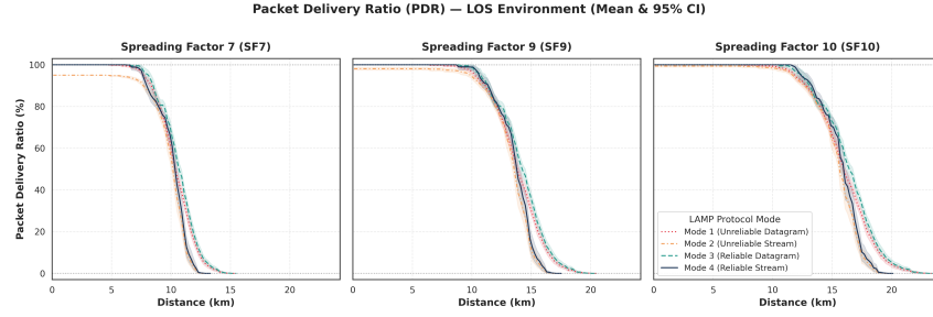
Fig. 5. Packet Delivery Ratio ( PDR_{app} %) as a function of distance across Spreading Factors (SF7, SF9, SF10) in Line-of-Sight (LoS) propagation. Solid lines denote mean delivery rates across 50 Monte Carlo trials; shaded ribbons represent 95% confidence intervals.
