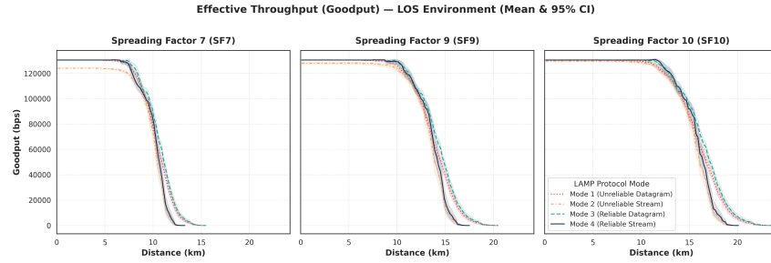
Fig. 6. Effective application-layer throughput (Goodput in bps) across Spreading Factors and LAMP operational modes in LoS. Shaded ribbons denote 95% confidence intervals across 50 Monte Carlo trials.
